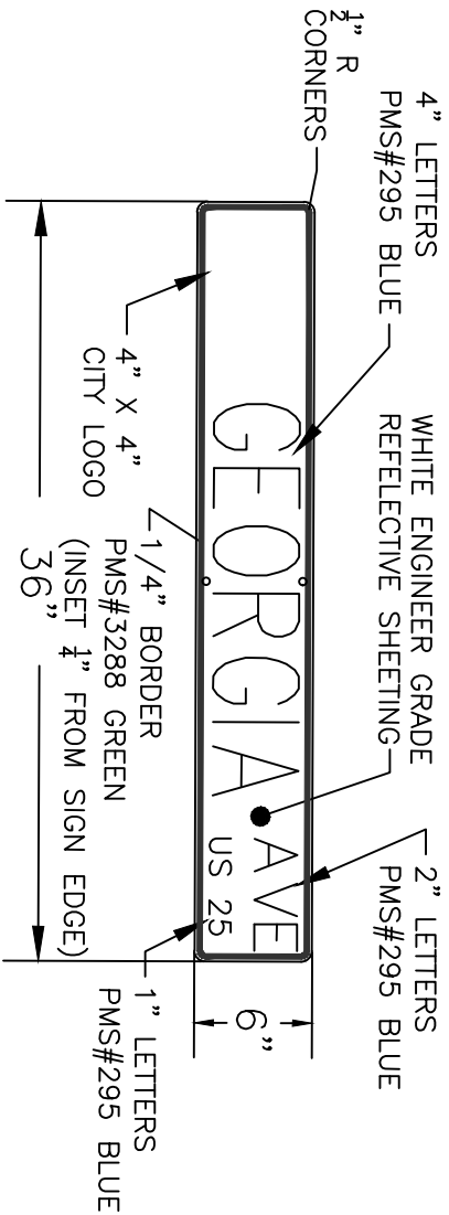
STANDARD STREET NAME SIGN
