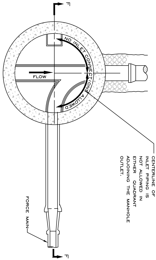
SECTIONAL PLAN
