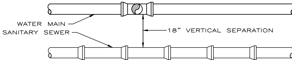
PROFILE VIEW
