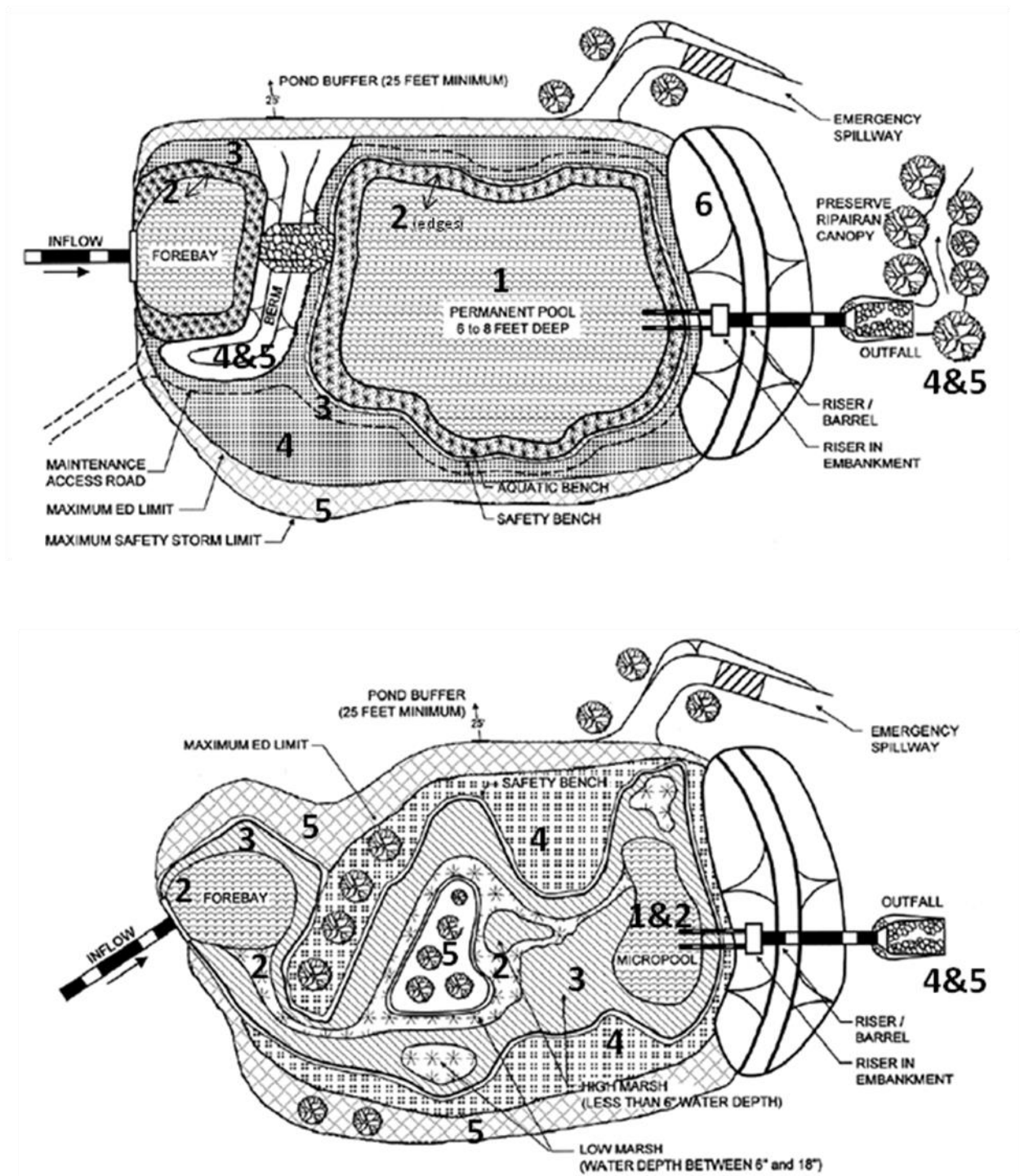
FIGURE C-1 HYDROLOGIC PLANTING ZONES
